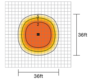
E-GP2L03CW fixture mounted at 12 feet with 0° tilt.
